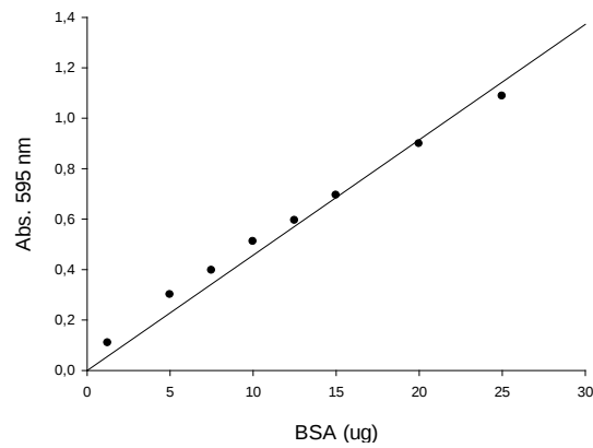
Figure 8 – Bradford microassay calibration curve with BSA. Linear regression, y = 0,0405x + 0,0859 ; r^2 = 0,998 .
