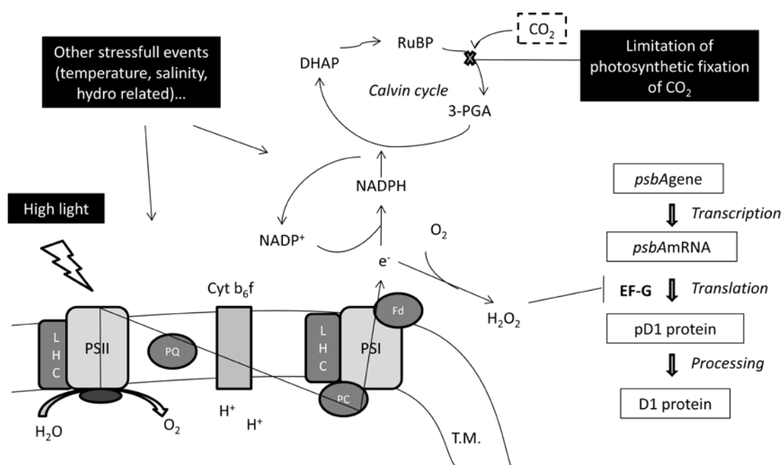
Figure 24 – Inhibition of repair by carbon limitation, adapted from Takahashi and Murata (2008). Other stressful events will cause further damage. DHAP is dihydroxyacetone phosphate; 3-PGA is 3-phosphoglyceric acid and RuBP is ribulose-1,5-bisphosphate.
