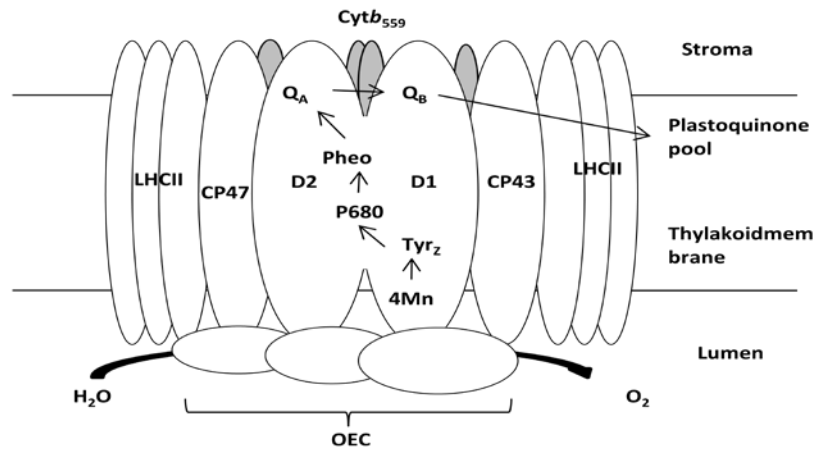
Figure 1 – Photosystem II architecture in thylakoid membranes, with reaction centres associated with the OEC and LHCII proteins, completed with electron trajectory (arrows). Cyt b_{559} – cytochrome b_{559} ; LHCII – light-harvesting complex II protein-pigment complexes; 4Mn – calcium manganese cluster associated with OEC- oxygen evolving complex; P680 – primary donor chlorophyll a ; Q_A – first acceptor plastoquinone; Q_B – second acceptor plastoquinone; Tyr Z – immediate electron donor tyrosine, from 4Mn to P680, in D1. D1, D2, CP43 and CP47 are proteins from the reaction centre. Adapted from Yamamoto et al. (2008).
