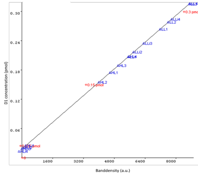
Figure 12 – Linear adjustment ( 3.44 \times 10^{-5} \cdot \text{Vol} + 0.0183 ; r^2 = 0.99 ) using standard D1 protein (Agrisera) densitometry of D1 protein [(INT*mm 2 )-Background] from P. tricornutum in experiment 1 in the four treatments: LL (low light, 40 \mu\text{mol photons.m}^{-2}.\text{s}^{-1} ); HL (high light, 1,250 \mu\text{mol photons.m}^{-2}.\text{s}^{-1} ); LLi (low light with lincomycin); and HLi (high light with lincomycin). Blue triangles are replicates of the various treatments and red crosses are standard concentrations of D1 (n=4).
